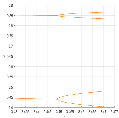
(c) 3.43 \leq r \leq 3.47 .
