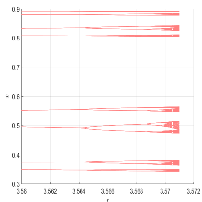
(e) 3.56 \leq r \leq 3.571 .
