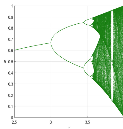
(f) 2.5 \leq r \leq 4 .
