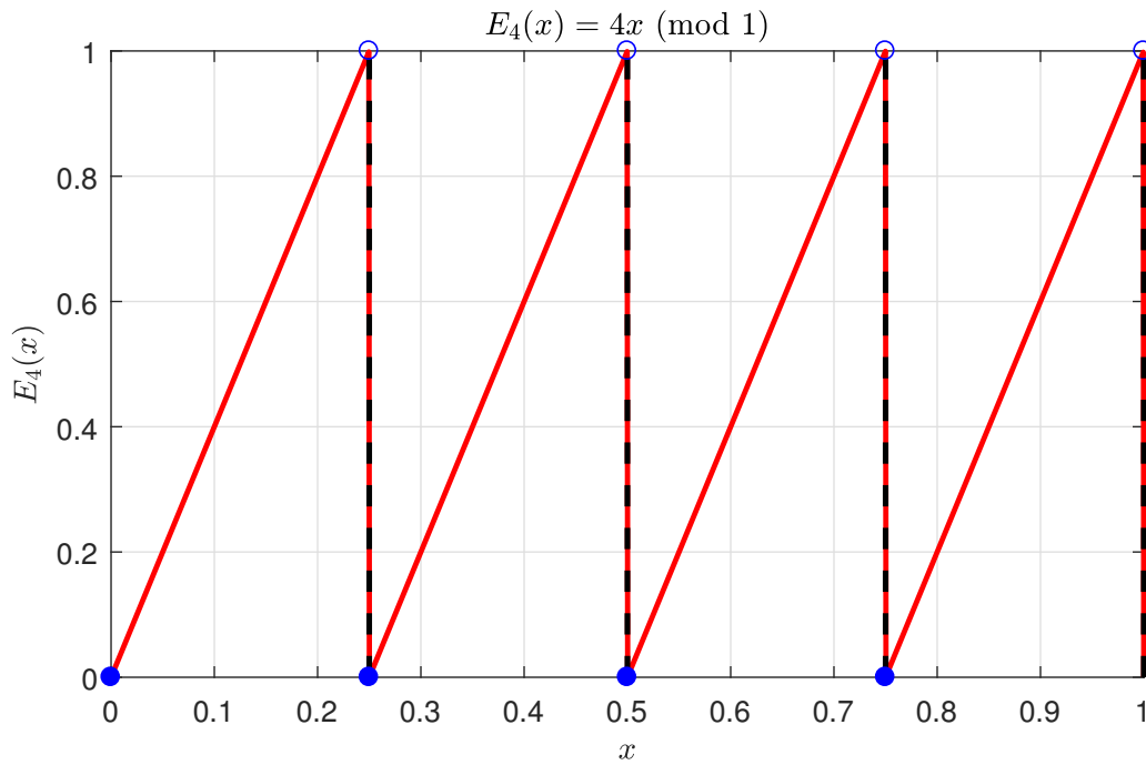
Figura 2.17: f(x) = E_4(x) .
