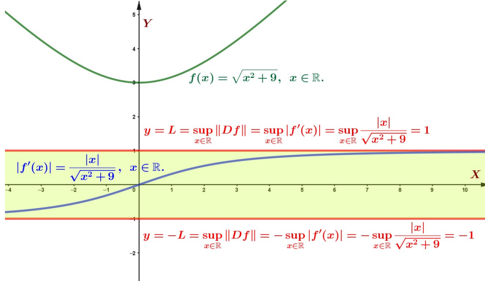
Figura 2.16: f(x) , f'(x) y L := \sup_{x \in \mathbb{R}} |f'(x)| = 1 .
