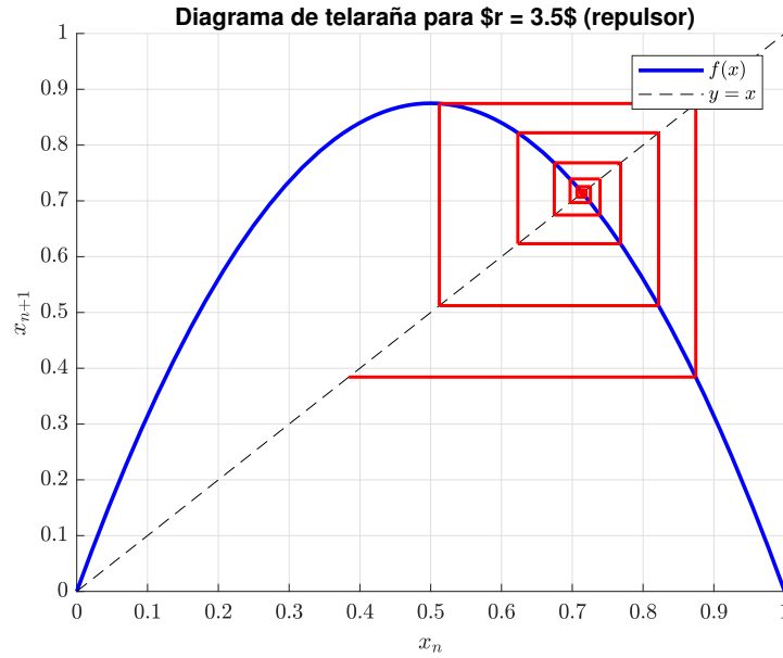
Figura 2.3: f(x) = rx(1 - x) , r = 3.5 (repulsor)
