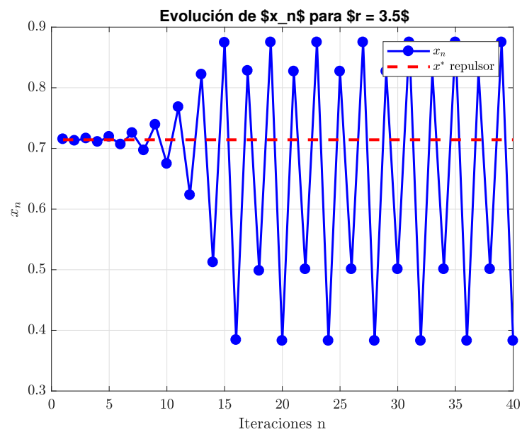
Figura 2.2: f(x) = rx(1-x) , r = 3.5 (repulsor)
