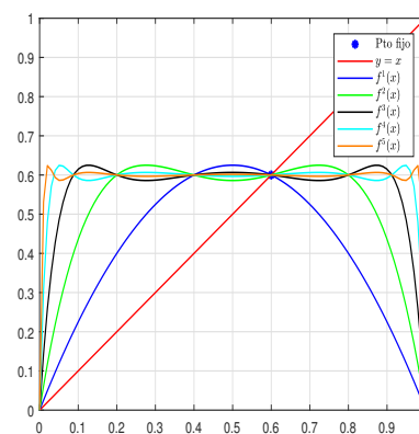
(f) n = 1, \dots, 5 .
