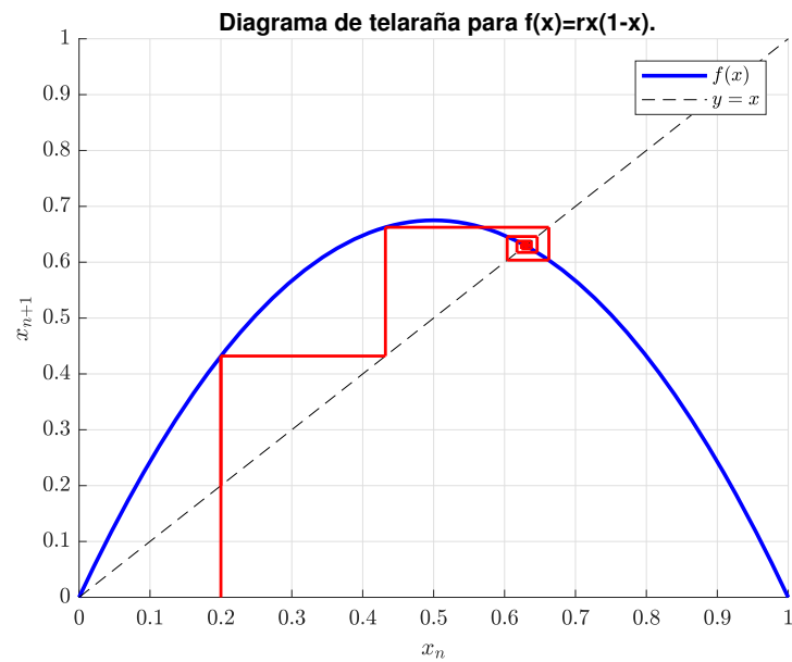
Figura 2.1: f(x) = rx(1-x) , x_0 = 0.2 , r = 2.7
