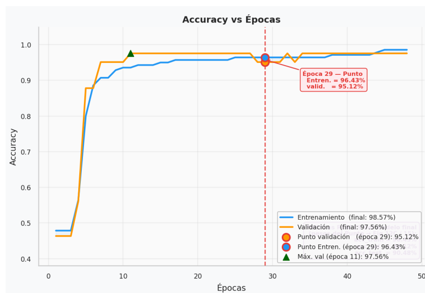
Figura 213 Accuracy vs. Épocas
