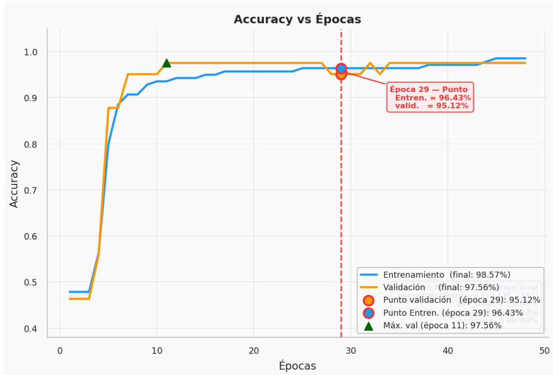
Figura 104 Accuracy vs. Épocas
