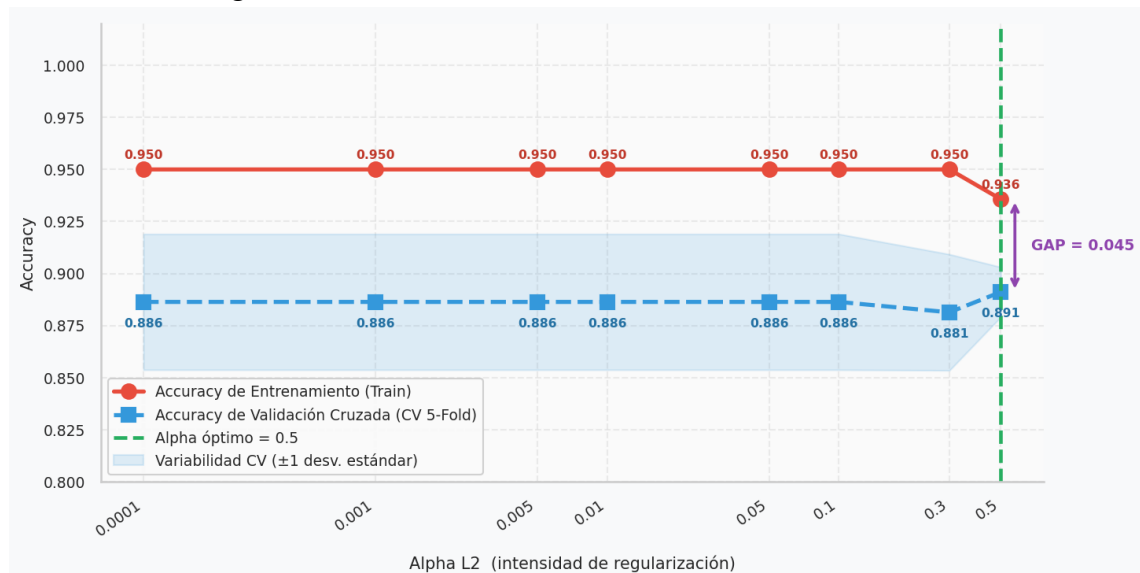
Figura 96 Accuracy vs. Alpha L2.
