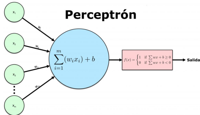
Figura 18 Red Neuronal Perceptron Simple.
