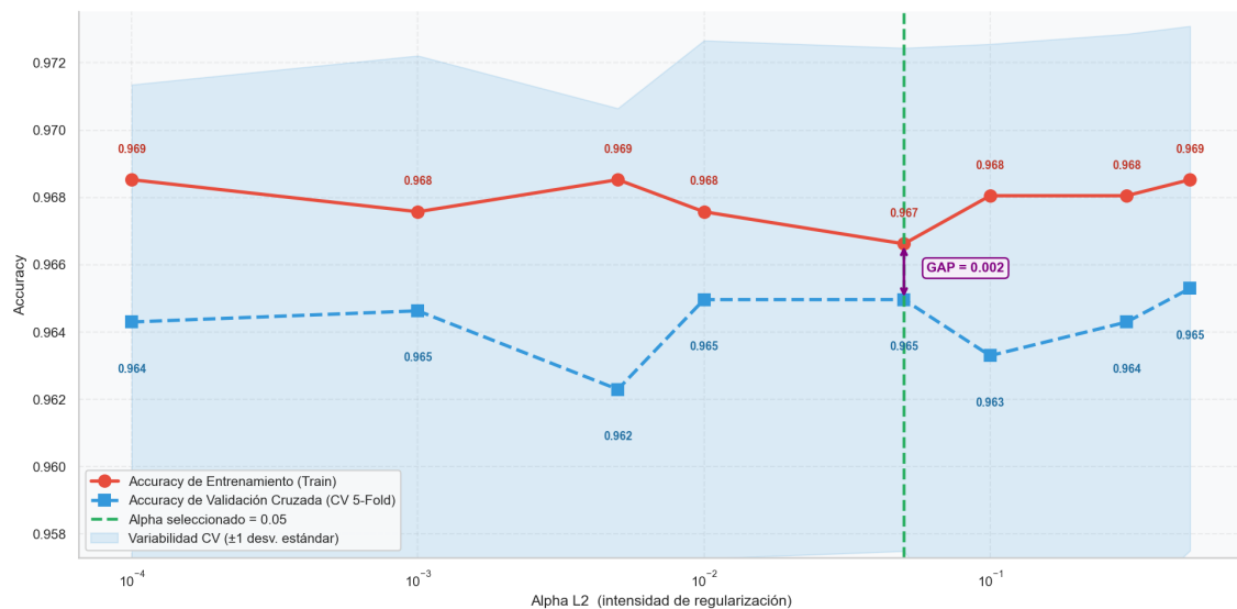
Figura 167 Accuracy vs Alpha L2.
